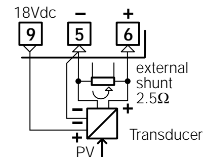
With 3 wire transducer
