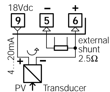
With 2 wire transducer
