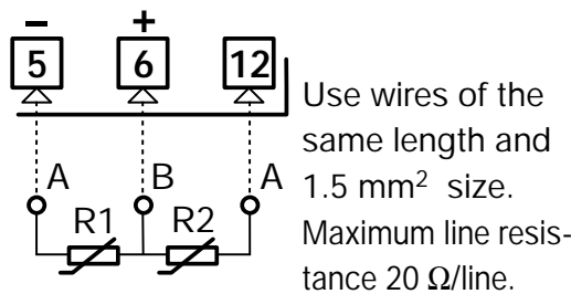
For ΔT (2 x RTD Pt100) Special
